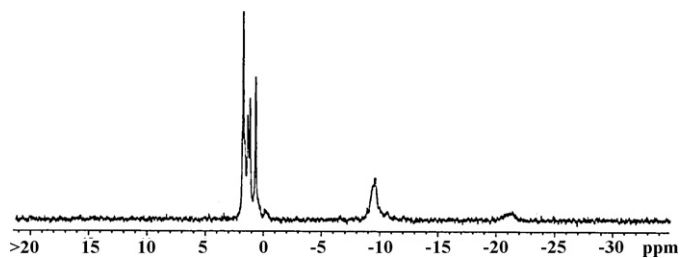
Fig. 2. ^{31}\text{P} NMR spectrum of the phosphated (1 → 3)- \alpha -D-glucan in \text{D}_2\text{O} .
